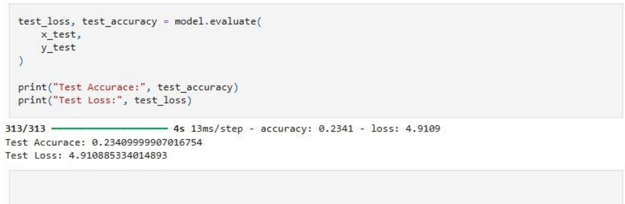
Figure 06: Performance evaluation of the non-quantized MobileNetV2 model.
